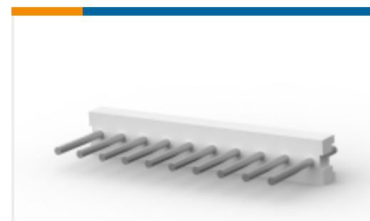
TE Part # 1-640384-0 10P MTA156 HDR ASSY STR RND SN
